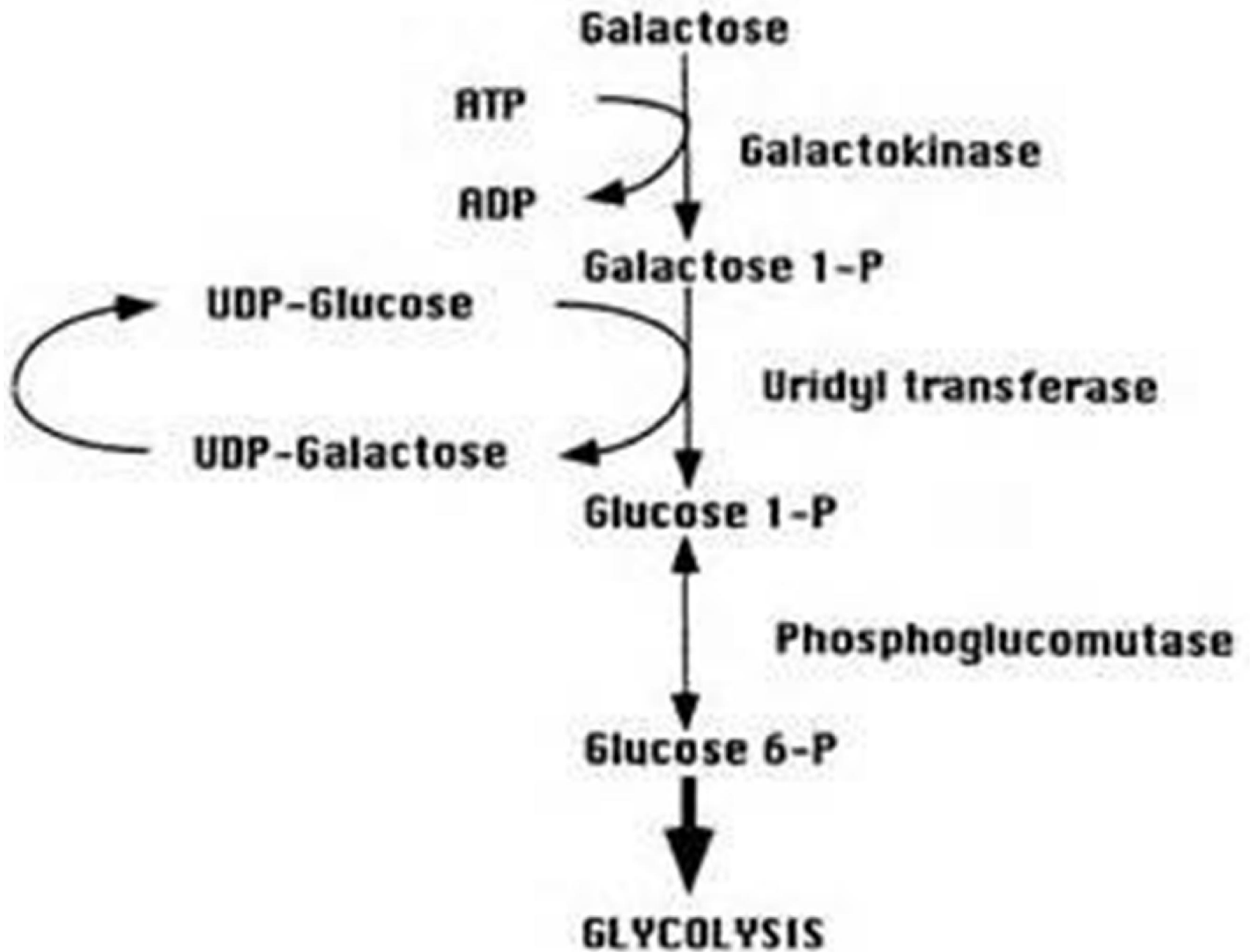
FIG 1: GALACTOSE METABOLISM
